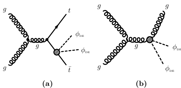
Figure 7. Schematic representation of representative production modes for the DE model for the Lagrangian effective operators (a) \mathcal{L}_1 and (b) \mathcal{L}_2 .
