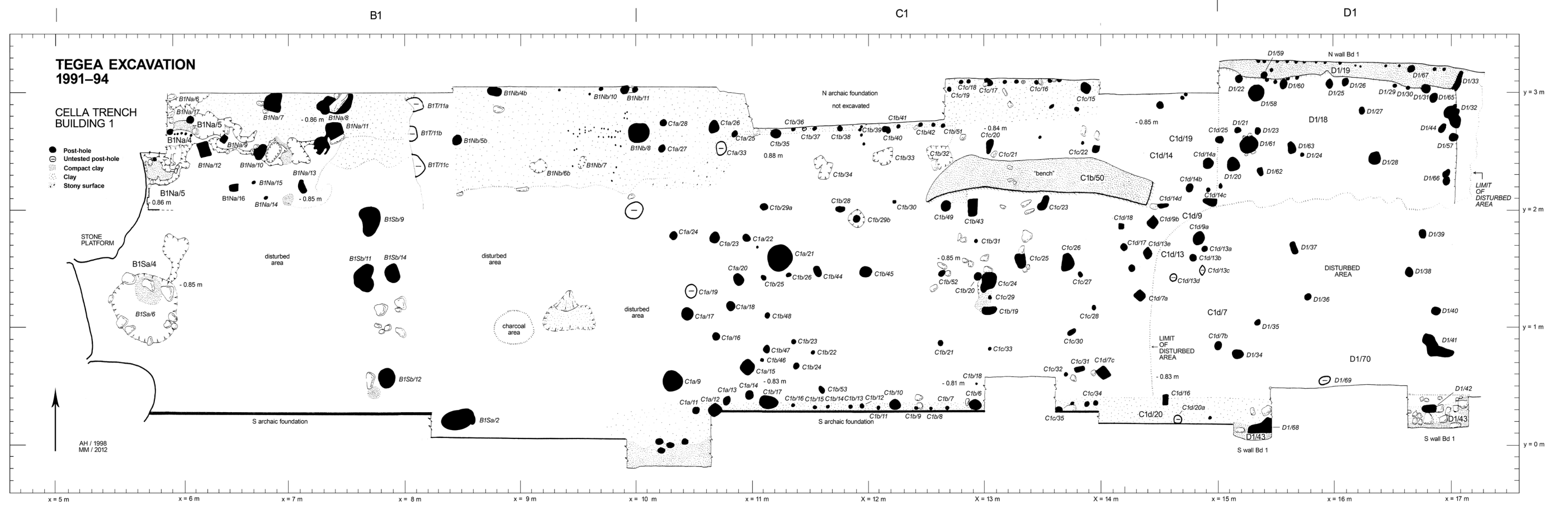
Plate 1. Building 1, plan of the remains. Scale 1 : 25. (Drawing: A. Hooton and M. Mauzy)
