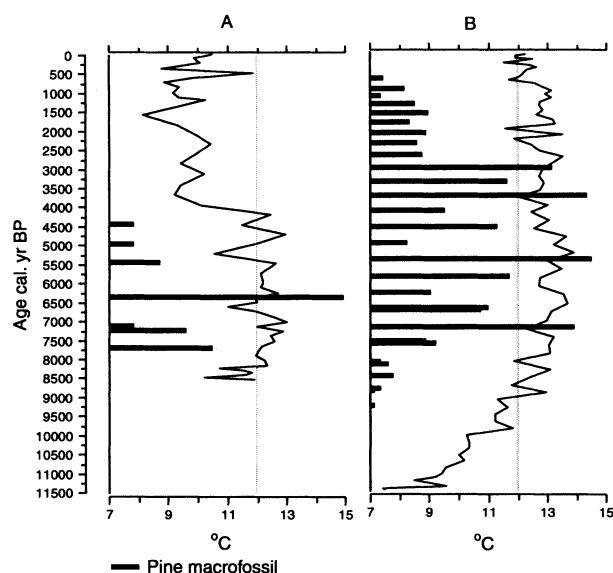
Figure 5 The inferred T_{jul} and the presence of pine macrofossils at (A) Trettetjørn and (B) Vestre Øykjamyrtjørn. A reference line is added at 12°C.
