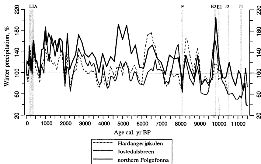
Figure 6 Holocene variations in winter precipitation in% compared to the present day calculated from Jostedalbreen, Hardangerjøkulen and northern Folgefonna based on the T_{jul} from Vestre Øykjamyrtjørn. 100% = 1961–90 normal. Some of the glacial events mentioned in the text are indicated by grey bar: LIA = 'Little Ice Age', F = Finse event; E1 = Erdalen event 1; E2 = Erdalen event 2; J1 = Jondal event 1; J2 = Jondal event 2 (see also Bakke et al. , 2005b).
