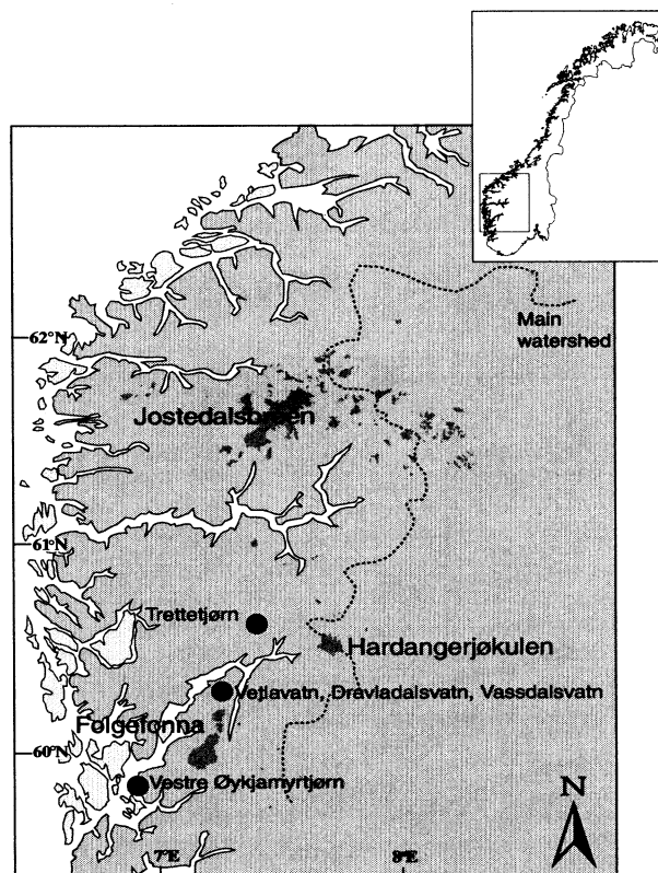
Figure 1 Map indicating the location of the lakes studied and the distribution of glaciers (shaded) in southern Norway.
