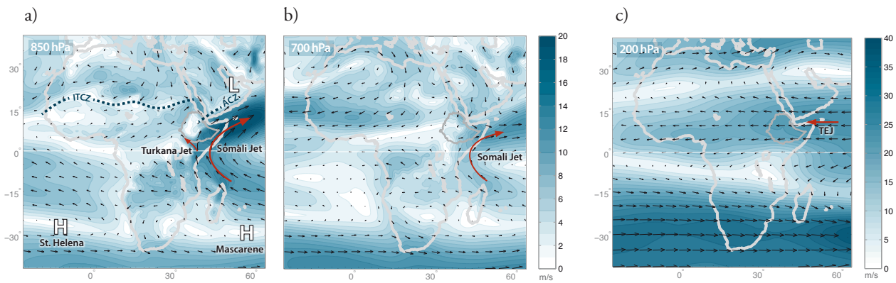
Figure 3 The atmospheric summer circulation over Africa
