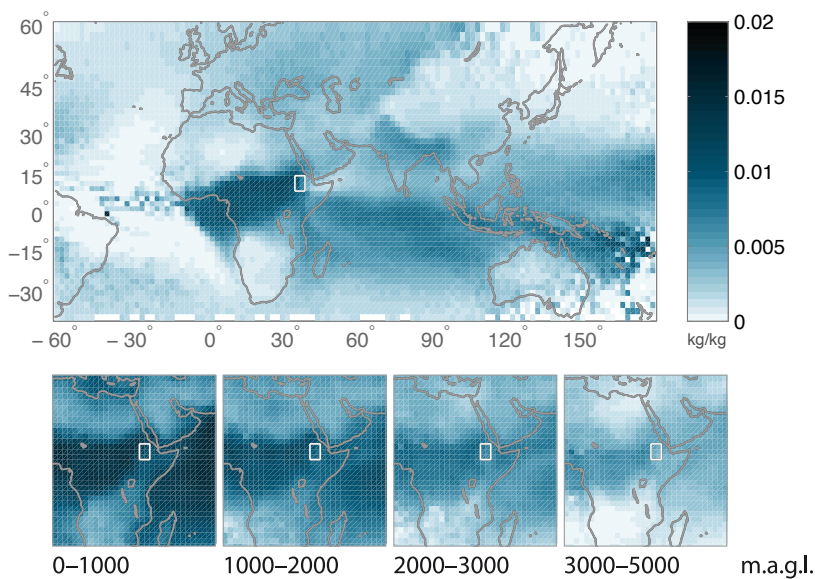
Figure 6 Humidity of air entering the northern Ethiopian highlands Mean specific humidity [kg/kg] of air 1–15 days before reaching 8–14 °N, 36–40 °E (white box) in July–August 1998–2008. Large map: All levels. Small maps: Same data classified by height [m.a.g.l.].
