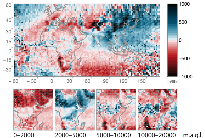
Figure 8 Vertical displacement of air
