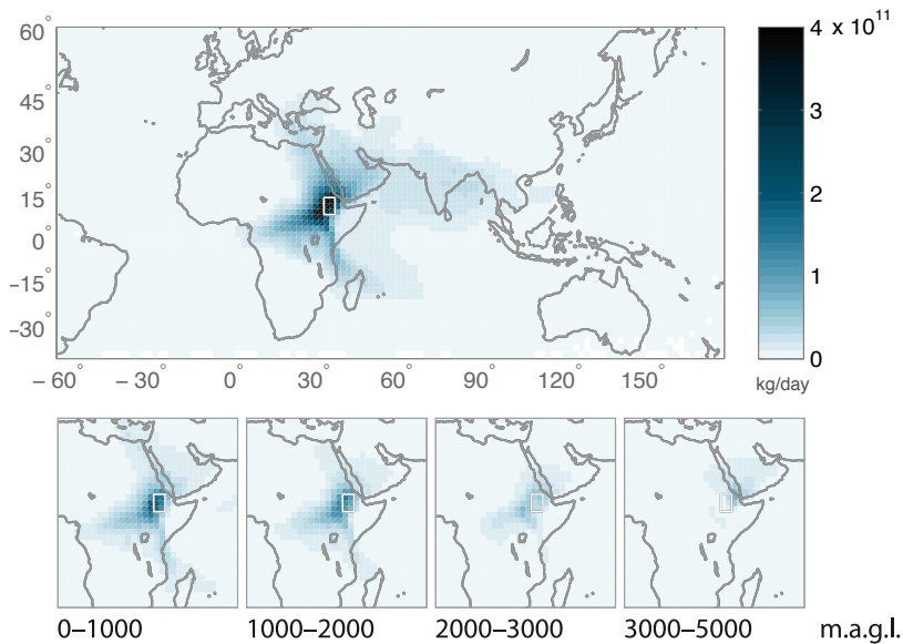
Figure 5 Transport of moisture into the northern Ethiopian highlands Mean daily moisture content [kg] of air 1–15 days before reaching 8–14 °N, 36–40 °E (white box) in July–August 1998–2008. Large map: All levels. Small maps: Same data classified by height [m.a.g.l.].
