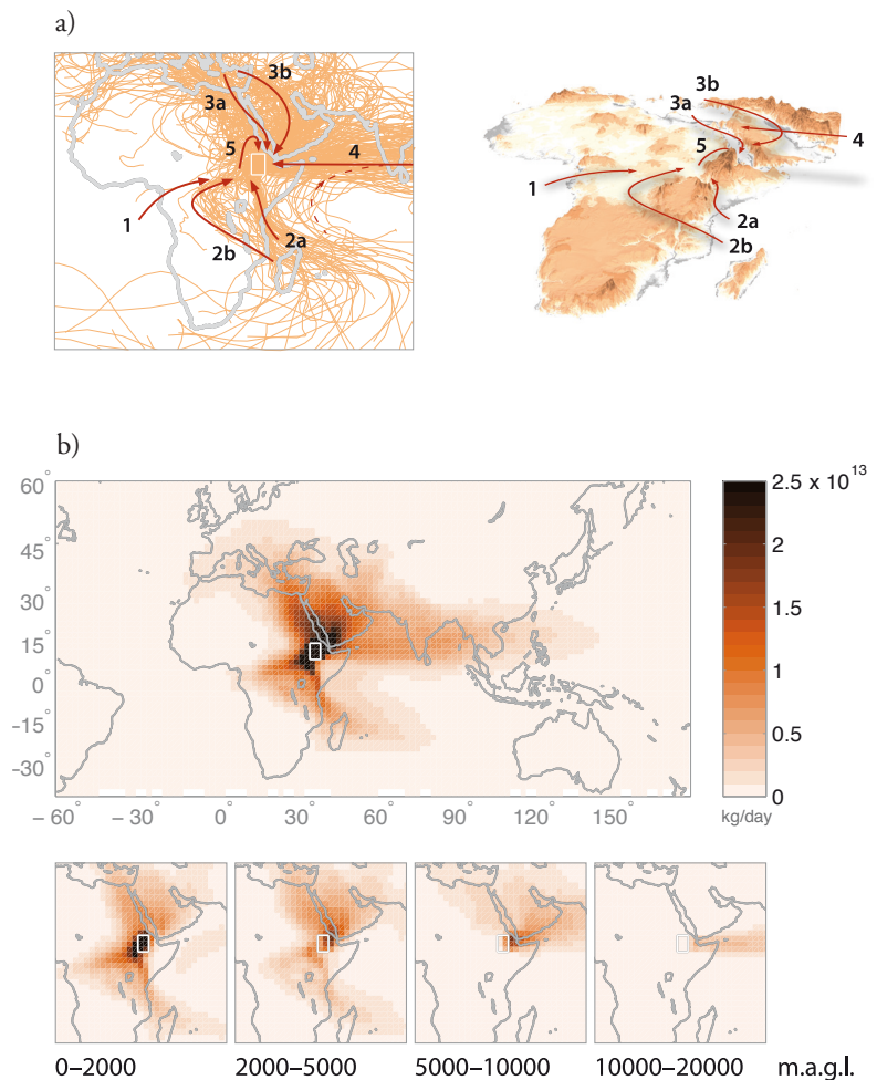
Figure 4 Transport of air into the northern Ethiopian highlands
