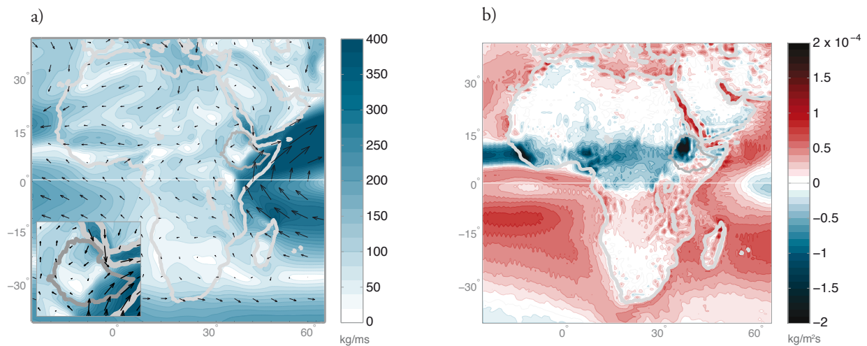
Figure 1 Moisture flow over Africa
