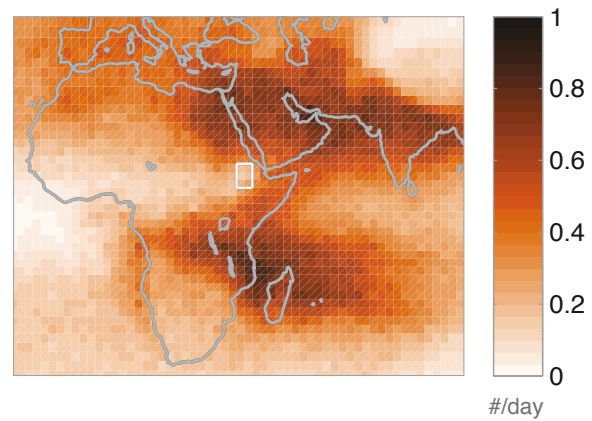
Figure 12 Location of air 20 days before Mean number of air parcels 20 days before reaching 8–14 °N, 36–40 °E (white box) in July–August 1998–2008.
