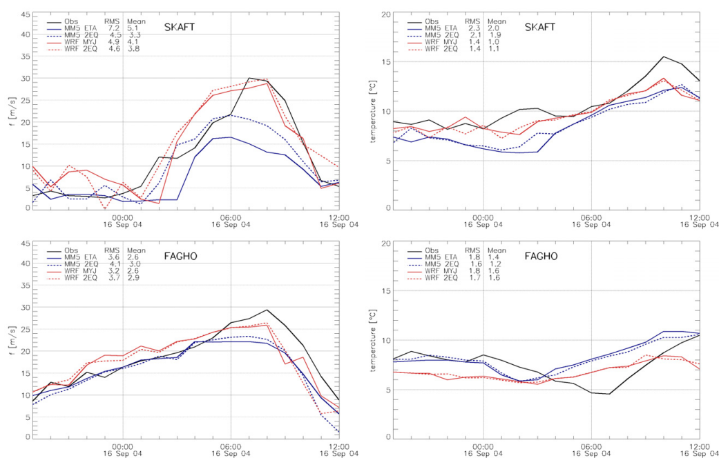
Fig. 5. Observed (solid black) and simulated (solid blue – MM5/ETA, blue dash – MM5/2EQ, solid red – WRF/MYJ, red dash – WRF/2EQ) 10 m wind speed [ \text{m s}^{-1} ] (left) and 2-m temperature [ ^{\circ} ] (right) at station SKAFT (WMO# 4172, top row) in the lee of Mt. Öræfajökull and at station FAGHO (bottom row).
