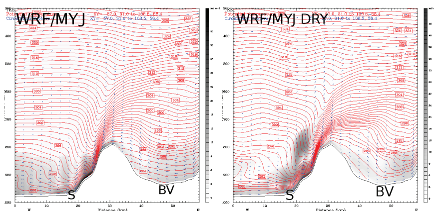
Fig. 14. Cross section along line AB (cf. Fig. 4) showing potential temperature (red lines) [K], wind along the cross section (blue arrows) [ \text{m s}^{-1} ] and turbulent kinetic energy (TKE) [J/kg] for WRF/MYJ (left) and WRF/MYJ DRY (right) at 16 September 2004, 06:00 UTC.
