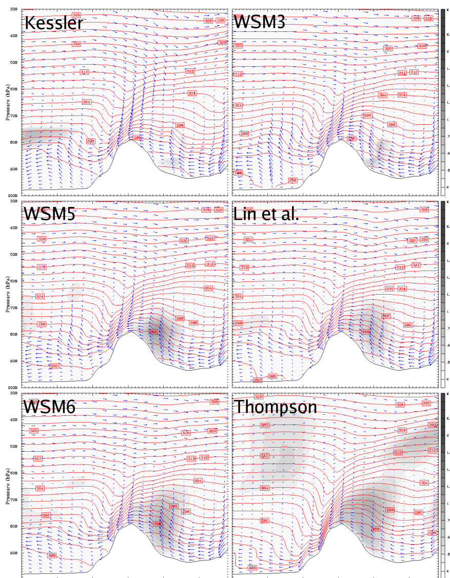
Fig. 9. Cross section along line AB (cf. Fig. 4) showing potential temperature (red lines) [K], wind along cross section (blue arrows) [ \text{ms}^{-1} ] and cloud water mixing ratio [g/kg] at 06:00 UTC 16 September 2004. micro-physics schemes are, from top left to bottom right: Kessler, WSM3, WSM5, Lin et al., WSM6 and Thompson.
