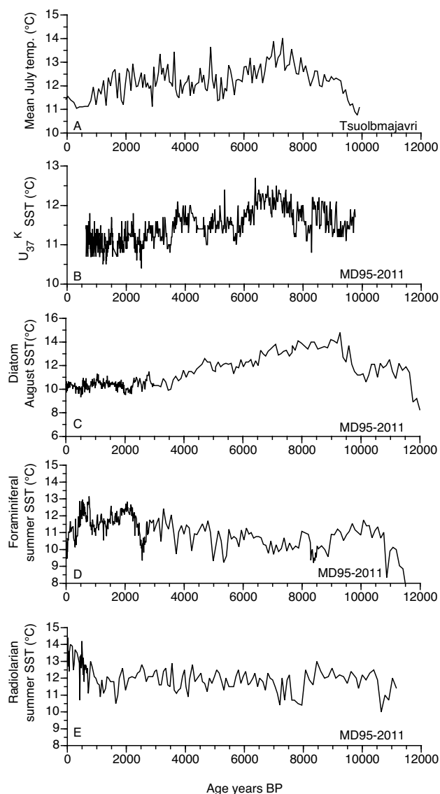
Fig. 6. (A) Mean July temperature based on pollen from Tsuolbmajavri, Finland (Seppä and Birks, 2001). (B) Alkenone derived sea-surface temperatures from the Vøring Plateau (MD95-2011) (Calvo et al., 2002; Jansen et al., 2008). (C) Diatom-based sea-surface August temperature estimates from MD95-2011 (Birks et al., 2002). (D) Foraminiferal-based transfer function sea-surface temperature estimates for summer (JAS) for MD95-2011 (Andersson et al., 2003; Risebrobakken et al., 2003; this study). (E) Radiolarian-based transfer function sea-surface summer temperature estimates for MD95-2011 (Dolven et al., 2002).
