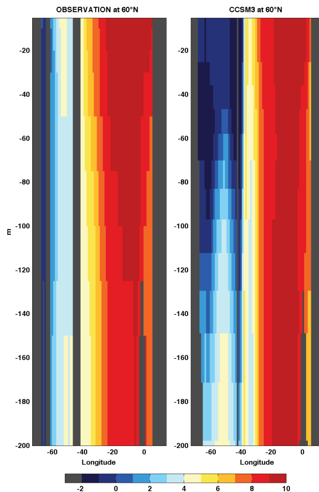
Fig. 2. Comparisons of annual temperature between CCSM3 and WOA98 at a transect 60^\circ\text{N} . NODC WOA98 data were provided by the NOAA/OAR/ESRL PSD, Boulder, Colorado, USA, from their Web site at http://www.esrl.noaa.gov/psd/ .
