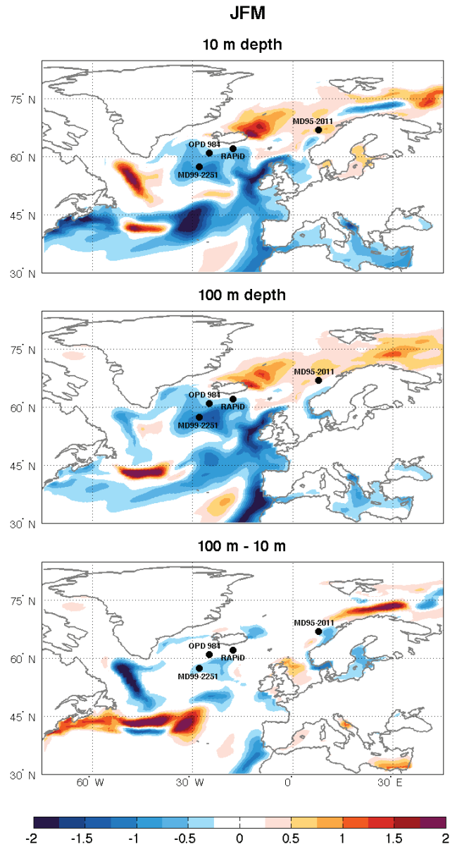
Fig. 10. 6k-0k CCSM3 model result for winter (JFM) temperature for 10 m and 100 m as well as the 6k-0k anomaly for the difference between 100 m and 10 m.
