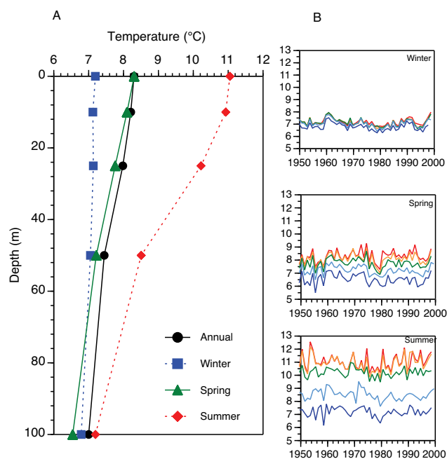
Fig. 7. (A) Seasonal and annual temperature averages for the last 50 years from Ocean Weather Station Mike in the upper 100 m of the water column. Averages are based on the temperature records presented in (B). From Nyland et al. (2006).
