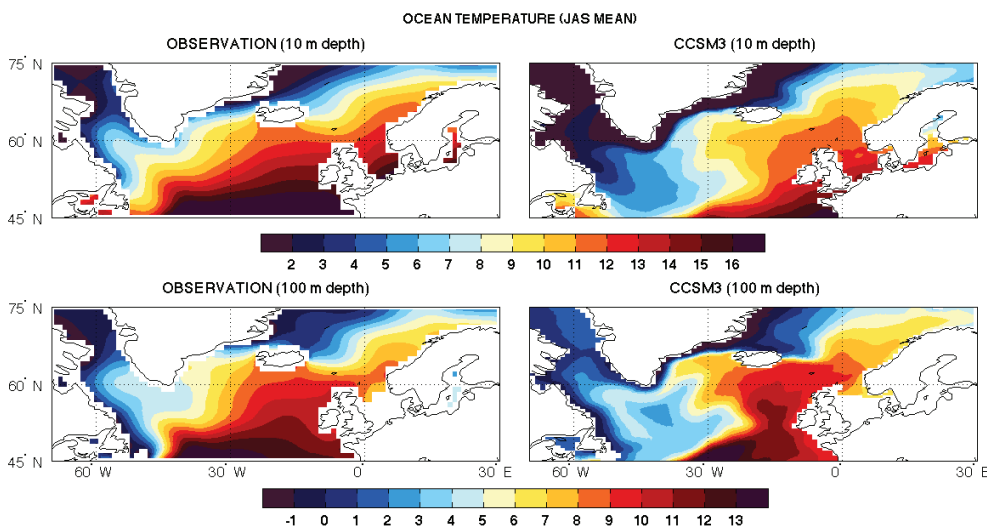
Fig. 5. Comparison of the mean July, August, and September temperature at 10 m and 100 m between CCSM3 and WOA98. NODC WOA98 data were provided by the NOAA/OAR/ESRL PSD, Boulder, Colorado, USA, from their Web site at http://www.esrl.noaa.gov/psd/ .
