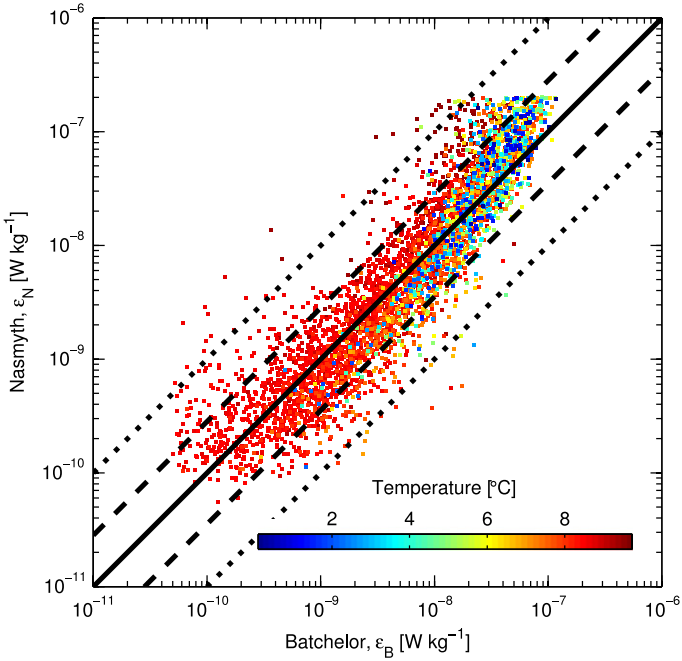
Fig. 12. Comparison of dissipation rates of TKE derived from the Batchelor fits ( \varepsilon_B ) and the shear probes (Nasmyth, \varepsilon_N ). Markers are color coded for temperature. The solid line represents a one-to-one agreement, the dashed and dotted lines mark deviations of factors 2.8 and 10, respectively.
