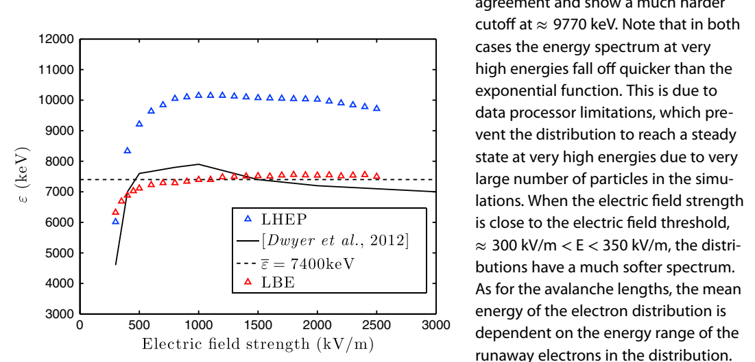
Figure 5. The mean energy of runaway electrons in an RREA with respect to electric field strength. The red and blue triangles again indicate the LBE results and the LHEP results, respectively. They are compared to the continuous black line, which represents the mean energies found by Dwyer [Dwyer et al. , 2012, Figure 3]. The dashed line represents the average mean energy, \bar{\epsilon} = 7400 \text{ keV} found from LBE results.
