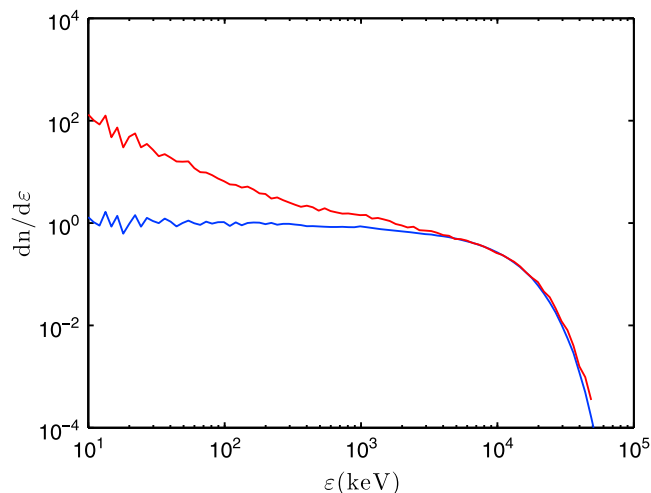
Figure 10. The energy distribution of RREAs simulated in an electric field of 400 kV/m. The red graph indicates the time-dependent simulation results, and the blue graph indicates the distance-dependent results.
