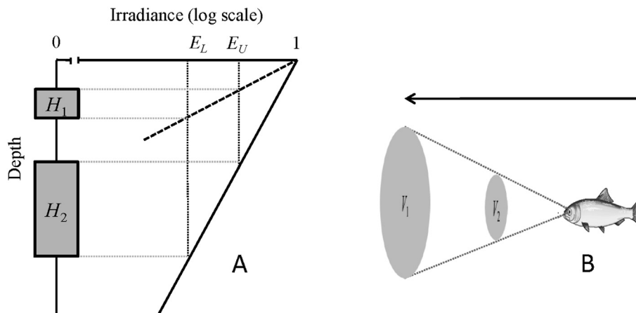
Fig. 6. The K - and c -effects on light sensitive organisms. Secchi depth shoaling is associated with increase in c and K (see Eq. (1)) A: An increase in the attenuation of downwelling irradiance from K_2 (solid line) to K_1 (broken line) shallows and narrows the habitat from H_2 to H_1 for an organism with a preference for a certain range of illumination. This range is here indicated by an upper ( E_U ) and a lower ( E_L ) irradiance level. B: An increase in the beam attenuation coefficient ( c ) reduces the visual area from V_1 to V_2 for a cruising predator.
