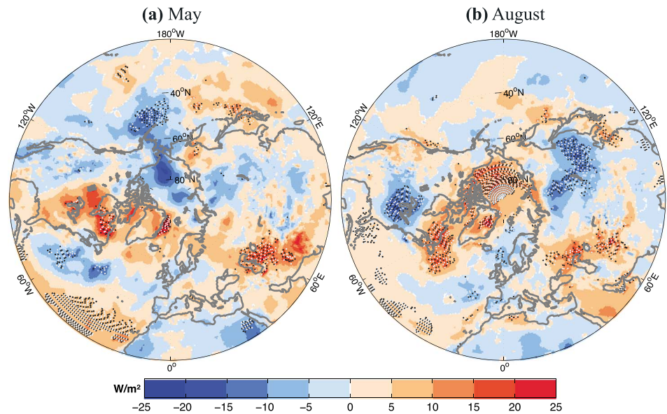
Figure 9. Incoming surface longwave radiation composites for HMR minus LMR months for (a) May and (b) August 1979–2013. Positive direction is downward. Alternating black and white dots mark regions of significant difference at a 95% confidence level.
