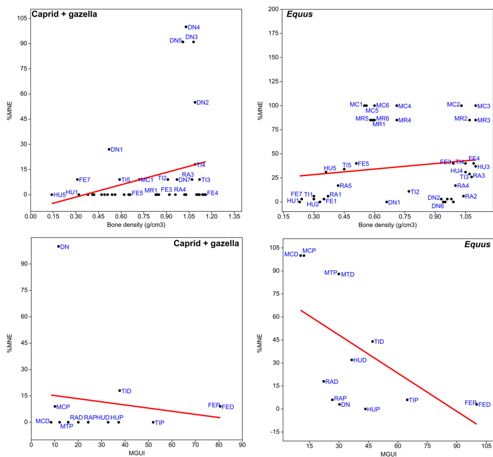
Fig. 8 Caprid + Gazella and equid high-survival element %MNE vs. bone mineral density ( BMD_2 ; g/cm^3 ) and the modified general utility index (MGUI). Full forms of abbreviations and raw data are provided in Supplementary Tables 11 and 12. Bone mineral density data for equids and wildebeest from Lam et al. (1999). Modified general utility data from Metcalfe and Jones (1988)
