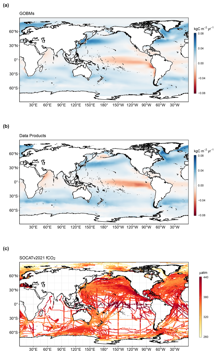
Figure B1. Ensemble mean air–sea \text{CO}_2 flux from (a) global ocean biogeochemistry models and (b) f\text{CO}_2 -based data products, averaged over 2011–2020 period ( \text{kgC m}^{-2} \text{yr}^{-1} ). Positive numbers indicate a flux into the ocean. (c) Gridded SOCAT v2021 f\text{CO}_2 measurements, averaged over the 2011–2020 period ( \mu\text{atm} ). In (a) model simulation A is shown. The data products represent the contemporary flux, i.e. including outgassing of riverine carbon, which is estimated to amount to 0.615 \text{ GtC yr}^{-1} .
