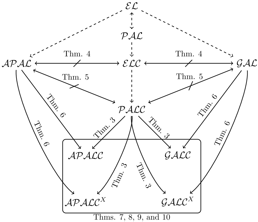
Fig. 10 Overview of the expressivity results. An arrow from \mathcal{L}_1 to \mathcal{L}_2 means \mathcal{L}_1 \leq \mathcal{L}_2 . If there is no symmetric arrow, then \mathcal{L}_1 < \mathcal{L}_2 . This relation is transitive, and we omit transitive arrows in the figure. An arrow from \mathcal{L}_1 to \mathcal{L}_2 is crossed-out, if \mathcal{L}_1 \not\leq \mathcal{L}_2 . Dashed arrows depict results known from literature, and solid arrows show the results proven in this paper. All languages in the rounded rectangle are pairwise incomparable
