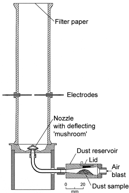
Figure 1. Cross-section of the dust dispersion system and explosion chamber. The air blast is generated by emptying a 50 cm 3 pressurised air reservoir, fitted with a solenoid valve, upstream of the dust reservoir. Further details are given in [7].
