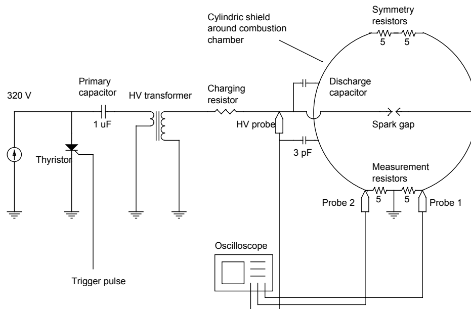
Figure 2. Schematic layout of the new spark discharge circuit and integrated spark energy measurement system. By triggering of the thyristor, sparks that can be synchronised with the dust dispersion are generated. Further details about the generator are given in [8].
