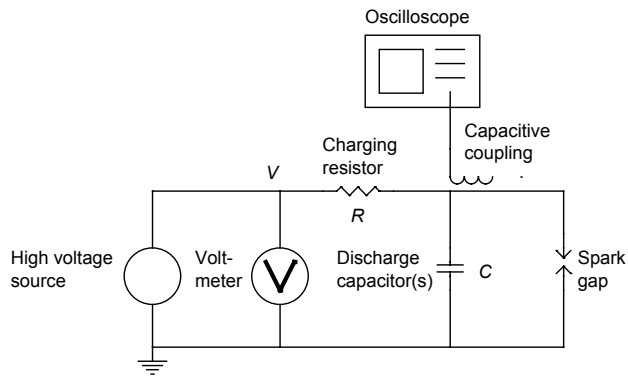
Figure 3. Schematic layout of the electric discharge circuit used when the explosive dust cloud itself triggers the spark discharge. The voltmeter is integrated in the high voltage source, measuring the output voltage V . The capacitive coupling is simply a wire twisted around the electrode, to ensure that the presence of a spark is recorded by the oscilloscope. Further details are given in [7].
