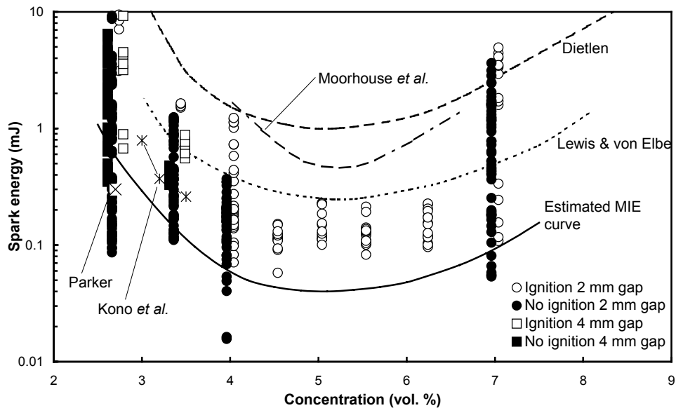
Figure 4. Minimum ignition energies for propane/air mixtures as a function of propane concentration. The white data points indicate ignition and the black no ignition, with 2 mm electrode gap represented as circles and 4 mm gap as squares. The solid line is an estimated MIE. Literature values are added [5, 11-14].
