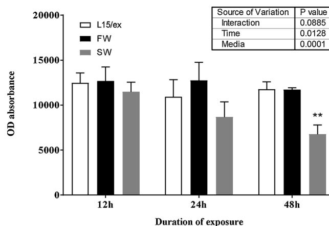
Fig. 1. Viability of RTgutGC cells (measured with Alamar blue assay) exposed to FW (black bar) and SW (grey bar) experimental media relative to L15/ex (white bar) as reference medium. Data are represented as mean \pm SD ( n = 3 ) of 12, 24 and 48 h exposure periods. Two-way ANOVA showed significant effect of both media composition ( P < 0.01 ) and time ( P < 0.05 ). Asterisk (*) indicates significant difference at each time point as obtained through Tukey's multiple comparison test (**, P < 0.01 ). (For interpretation of the references to colour in this figure legend, the reader is referred to the web version of this article).
