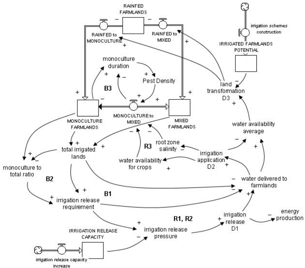
Figure 10. Causal loop diagram: irrigation release, irrigation application, land transformation, and environmental factors.
