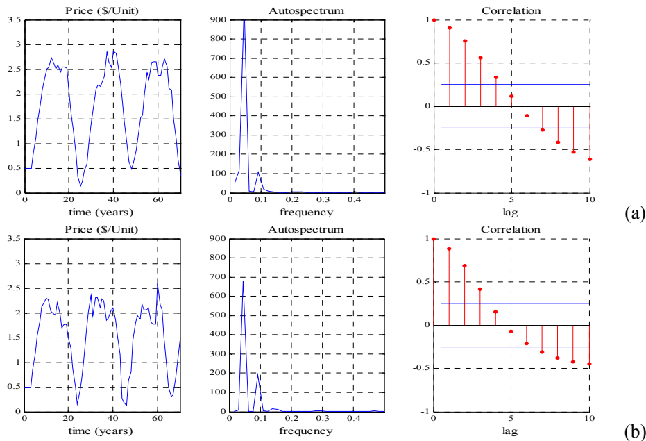
Figure 4. Simulated prices of the experimental market with noise for parameters set 1 (a) and set 2 (b). Both series have the autospectrum (performed with the last 64 data) and autocorrelation (horizontal lines are the 95% confidence bounds).
