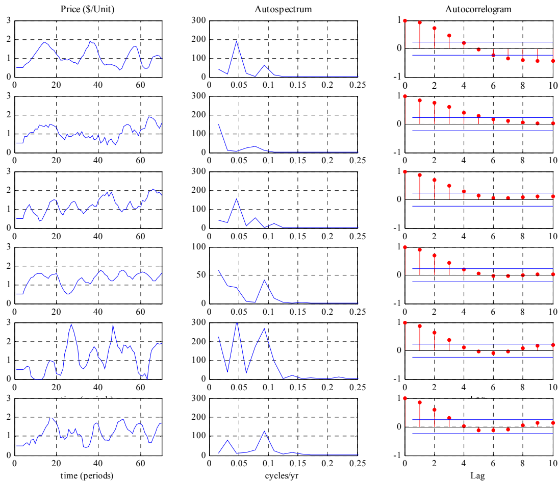
Figure 5. Realized prices in the six experimental markets, autospectrum and autocorrelations. Autospectrums are based on the last 64 data points of the series, and autocorrelations present the 95% confidence bounds (horizontal lines).
