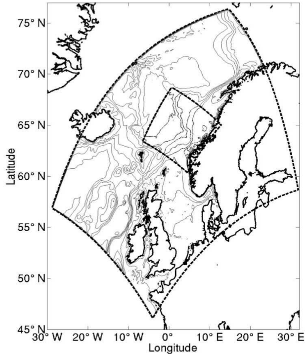
Fig. 1. The model domains of MEDIUM and FINE are shown, with the bathymetry in the area as contourlines.
