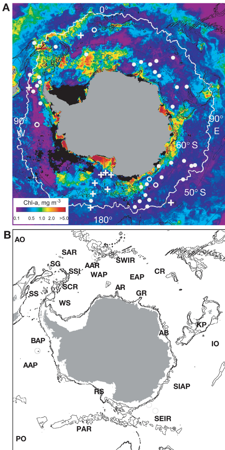
Fig. 2. (A) Satellite image of the Southern Ocean showing distribution of chl a (mg m -3 ) in surface waters during January and February 2000. Data are derived from the Sea-viewing Wide Field-of-view Sensor (SeaWiFS, McClain et al. 1998) using the standard OC4v2 chlorophyll algorithm (O'Reilly et al. 1998, 2000). The jagged white line is the 4°C isotherm, which is the approximate location of the Polar Front. Areas shown in black have insufficient data due to ice cover or to open waters with extensive cloud cover. Major bathymetric features (obtained from the ETOPO2 data base) are shown by the isobaths (thin black lines) for 2000, 2500, and 3000 m depths. The following shipboard acquired data have been added to the chl a image: locations where deep chl a maxima have been reported (white circles); locations in low chl a regions, where dissolved Fe concentrations have been reported (white crosses); and locations where both deep chl a maxima and dissolved Fe concentrations have been reported (white rings). Many of the symbols represent multiple stations; in these cases, the symbols shown occupy locations central to the reported stations. The coordinates and references for the chl a and Fe data are listed in Table 1. (B) Identification of land and bathymetric features shown in the upper panel; Scotia Sea (SS), the South Scotia Ridge (SCR), Weddell Sea (WS), South Georgia (SG), Atlantic Ocean (AO), South Sandwich Islands (SSI), South Atlantic Ridge (SAR), America Antarctic Ridge (AAR), Weddell Abyssal Plain (WAP), Astrid Ridge (AR), Southwest Indian Ridge (SWIR), Enderby Abyssal Plain (EAP), Gunnerus Ridge (GR), Conrad Rise (CR), Amery Basin (AB), Kerguelen Plateau (KP), Indian Ocean (IO), South Indian Abyssal Plain (SIAP), Southeast Indian Ridge (SEIR), Pacific Antarctic Rise (PAR), Ross Sea (RS), Pacific Ocean (PO), Amundsen Abyssal Plain (AAP), and Bellingshausen Abyssal Plain (BAP)
