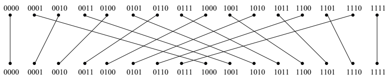
FIGURE 4.13: The perfect shuffle permutation of 2^4 elements. The new positions are obtained by cyclic shifts of the binary representations of the old positions. Hence 4 = \log_2 2^4 -step interconnection of this pattern with itself brings each element back to its original position.
