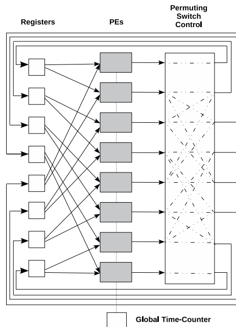
FIGURE 6.7: The schematic overview of a DDA-based shuffle network performing bitonic sorting of 2^3 inputs. (The dataflow is now identical with the direction of the arrows.)
