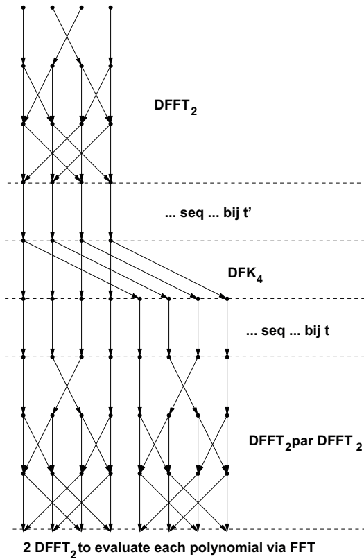
FIGURE 7.4: The structural composition of the DDA underlying the multiplication of polynomials with degree n_1 and n_2 such that n_1+n_2 < 4 .
