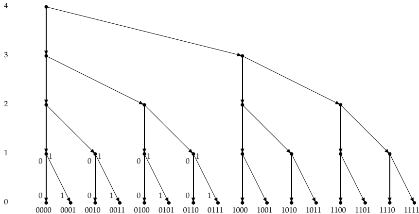
FIGURE 4.10: Binary tree DDA of height 4.
