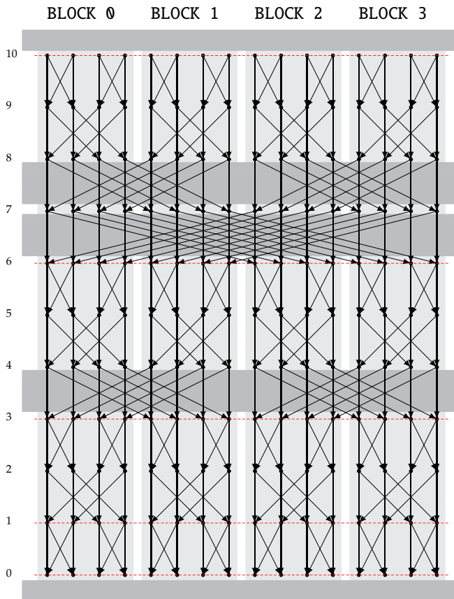
FIGURE 6.4: Bitonic sort DDA for 2^4 inputs, embedded into NVIDIA's CUDA programming model, executed by 4 kernel invocations, each consisting of 4 blocks of threads.
