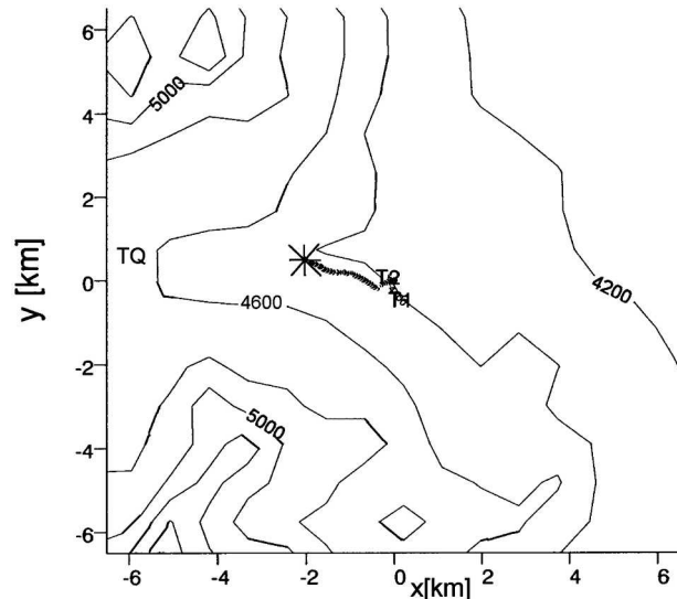
FIG. 14. Terrain and theodolite basis T_1\text{--}T_2 near Tambo Quemado (TQ). Also shown is the track of the balloon released at 1500 LST 19 Aug; final balloon height above starting point is 1779 m. Contour interval 200 m; star: end of trajectory.
